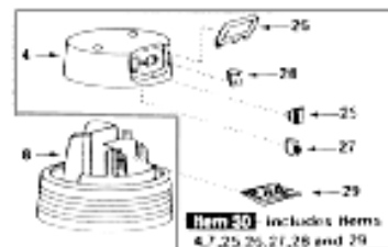
Detail Drawing A
