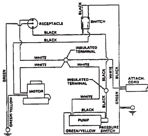
WIRING DIAGRAM - C3005-100
